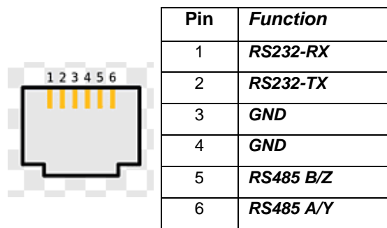
Serial Port Pinout
