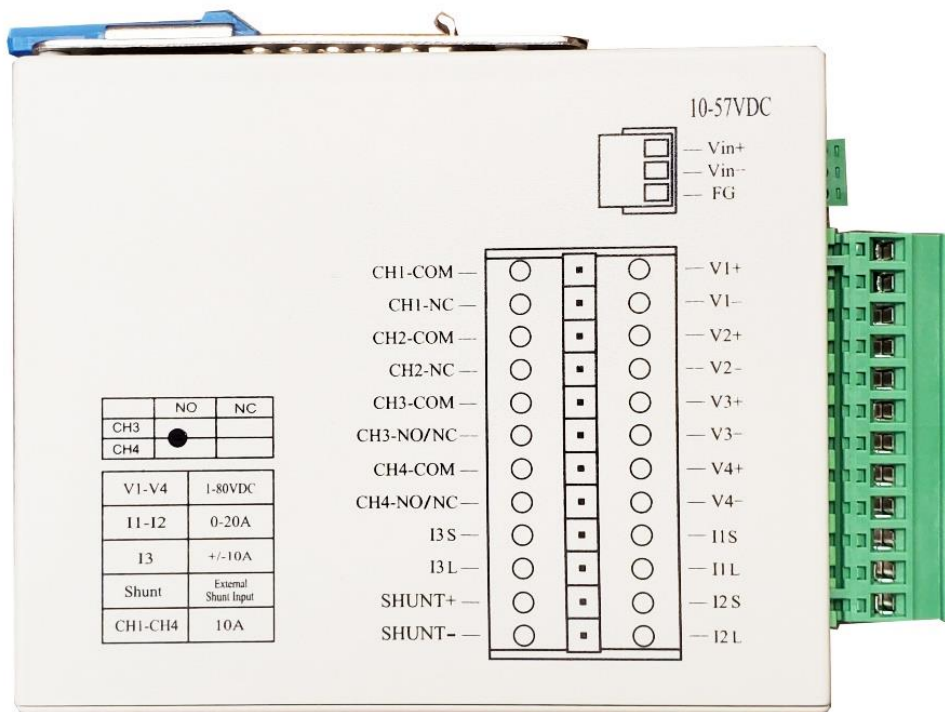
TPDIN® Connector Pinout
