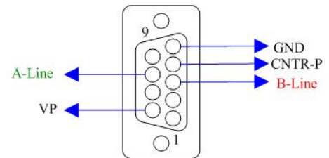
Female D-Sub Connector
