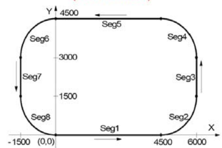
Continuous interpolation
